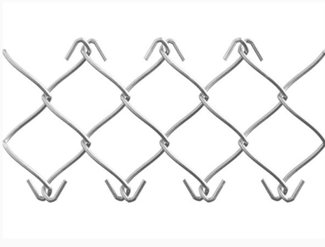
Chain Link Fence With Knuckle-Knuckle Selvage
