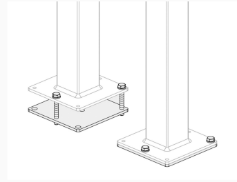
Ground Counterplate
