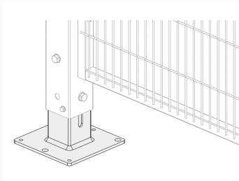
Adjustable Baseplate
