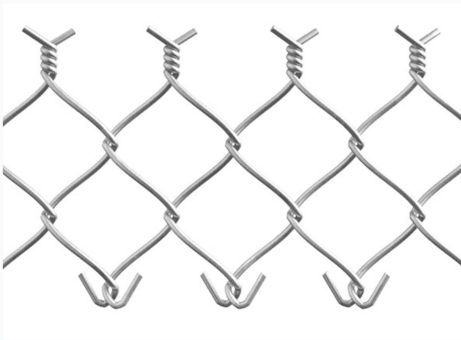
Chain Link Fence With Knuckle-Twist Selvedge
