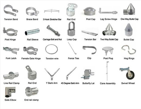
Chain Link Fence Components & Accessories
