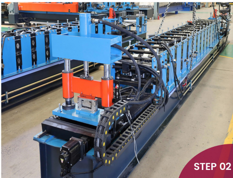
Pale Profile Forming
