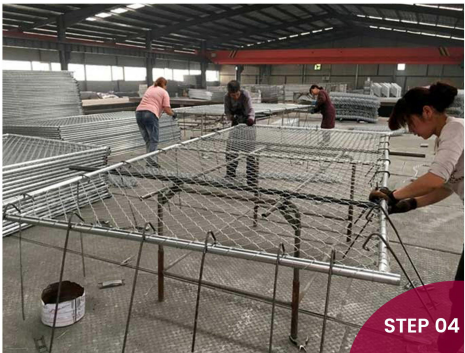
Chain Link Fence and Frame Assembly
