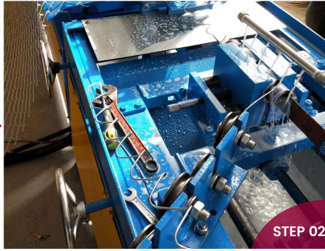
Teel Wire Straightening and Cutting
