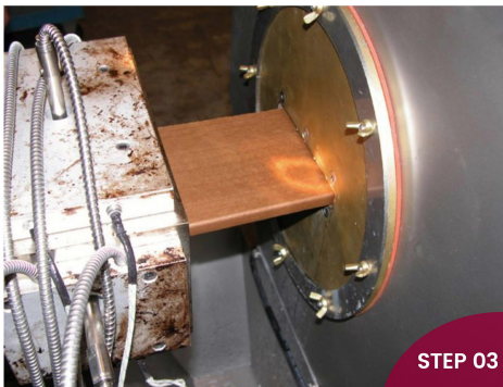
Extrusion Molding
