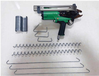
1.Welded Gabion Fitting
