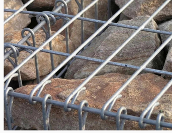
Hook Connection
