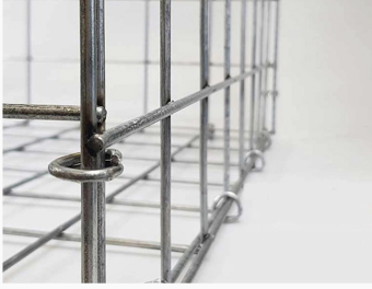
C-Rings Connection
