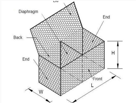
Specification Of Gabion Basket
